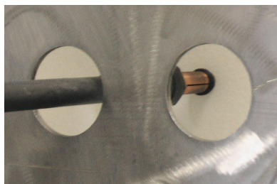
THRU-HOLE WELDING
